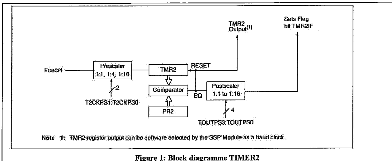
Figure 1: Block diagramme TIMER2
